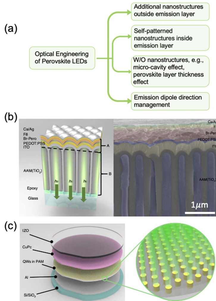
Figure 13. Optical engineering of PeLEDs. (a) General strategies of optical engineering of PeLEDs: (1) additional nanostructures outside EML; (2) self-patterned nanostructures inside EML; (3) w/o nanostructures, e.g. micro-cavity effect, perovskite layer thickness effect; (4) emission dipole direction management. (b) Example of additional nanostructures outside EML: nanodomes as light couplers and nanowire arrays as optical antennas. Reproduced from [158]. CC BY 4.0. (c) Example of self-patterned nanostructures inside EML, perovskite quantum wire arrays inside porous alumina membrane and the EML's effective refractive index is reduced. Reproduced from [163], with permission from Springer Nature.
