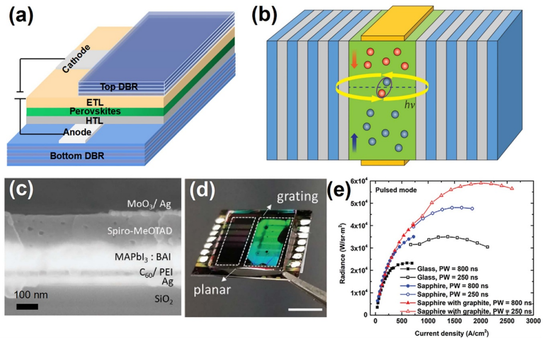
Figure 27. (a) The photons cycle in a direction perpendicular to the DBR layers. (b) Electrons (blue circles) and holes (red circles) are electrically injected from below and above, orthogonal to the cavity feedback, thereby minimizing optical losses. h\nu is the cavity photon. Reproduced from [273], with permission from Springer Nature. (c) Cross-sectional scanning electron microscope image of the full device stack. (d) Photograph of completed devices. Irrescence from the DFB grating is visible on the right half of the substrate, while the left half is not imprinted to serve as a planar control. The scale bar is about 1 cm. [269] John Wiley & Sons. © 2019 WILEY-VCH Verlag GmbH & Co. KGaA, Weinheim. (e) Radiance–current density curves of PeLEDs on glass or sapphire substrates, with or without a graphite heat spreader and copper heat sink, all driven in pulsed mode. [93] John Wiley & Sons. © 2020 WILEY-VCH Verlag GmbH & Co. KGaA, Weinheim.
