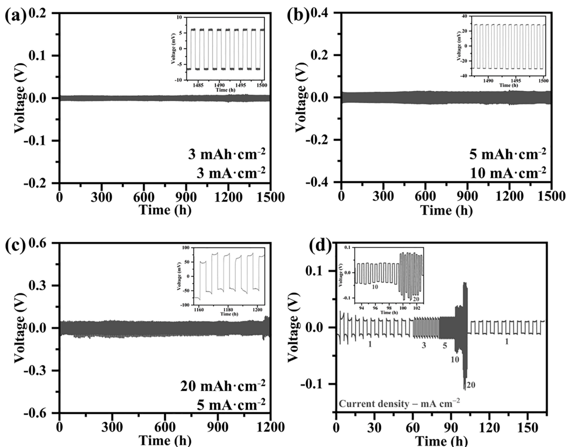
Fig. 5. Electrochemical symmetric cell performance of \text{Ti}_3\text{C}_2\text{Tx}/\text{CNT} NAFs// \text{Ti}_3\text{C}_2\text{Tx}/\text{CNT} NAFs at varying capacities and currents of (a) 3.0 \text{ mAh cm}^{-2} at 3.0 \text{ mA cm}^{-2} , (b) 5.0 \text{ mAh cm}^{-2} at 10.0 \text{ mA cm}^{-2} , and (c) 20.0 \text{ mAh cm}^{-2} at 5.0 \text{ mA cm}^{-2} ; each inset shows last few cycles. (d) The rate capability of \text{Ti}_3\text{C}_2\text{Tx}/\text{CNT} NAFs// \text{Ti}_3\text{C}_2\text{Tx}/\text{CNT} NAFs symmetric cell at a current of 1 – 20 \text{ mA cm}^{-2} ; inset shows rate performance at 10 and 20 \text{ mA cm}^{-2} .
