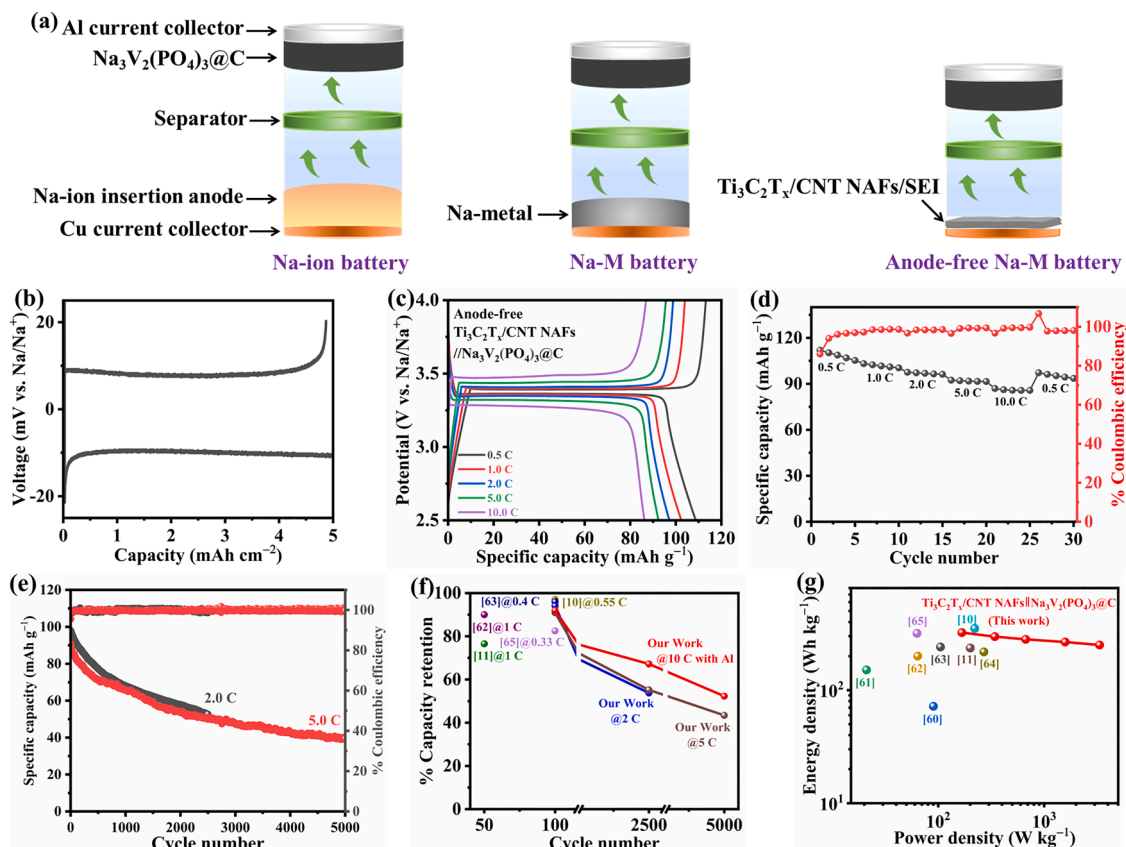
Fig. 6. (a) A schematic representation of distinctions between Na-ion, Na-M, and AFSMBs. (b) Preconditioning process of anode-free \text{Ti}_3\text{C}_2\text{T}_x/\text{CNT} NAFs/Na-SEI. Electrochemical full-cell performance of anode-free \text{Ti}_3\text{C}_2\text{T}_x/\text{CNT} NAFs/Na-SEI// \text{Na}_3\text{V}_2(\text{PO}_4)_3@C cell. (c) GCD plot and (d) rate capability plot at different C-rates of 0.5 C–10.0 C of the anode-free \text{Ti}_3\text{C}_2\text{T}_x/\text{CNT} NAFs/Na-SEI// \text{Na}_3\text{V}_2(\text{PO}_4)_3@C cell. (e) Cyclic stability plots of anode-free \text{Ti}_3\text{C}_2\text{T}_x/\text{CNT} NAFs/Na-SEI// \text{Na}_3\text{V}_2(\text{PO}_4)_3@C cells at 2.0 and 5.0 C. (f) Comparison of capacity retention of anode-free \text{Ti}_3\text{C}_2\text{T}_x/\text{CNT} NAFs/Na-SEI// \text{Na}_3\text{V}_2(\text{PO}_4)_3@C cells with previously reported anode-free full cells. (g) Ragone plot of anode-free \text{Ti}_3\text{C}_2\text{T}_x/\text{CNT} NAFs/Na-SEI// \text{Na}_3\text{V}_2(\text{PO}_4)_3@C full cell with previously reported \text{Na}_3\text{V}_2(\text{PO}_4)_3@C -based anode-less/anode-free SMBs.
