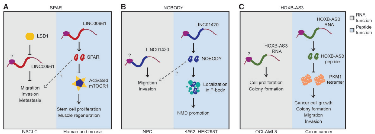
Figure 1. Cancer-related lncRNAs with functional peptides. Left side (gray box) of each figure shows the RNA function. (A) LINC00961 related to NSCLC. (B) LINC01420 related to NPC. (C) HOXB-AS3 transcript related to AML in OCI-AML3 cells. The right side (blue box) shows the functions for the peptides. (A) SPAR inhibiting mTORC1 activation. (B) NOBODY promoting NMD in K562 and HEK293T cells. (C) HOXB-AS3 peptide regulating PKM splicing and suppressing cancer growth.
