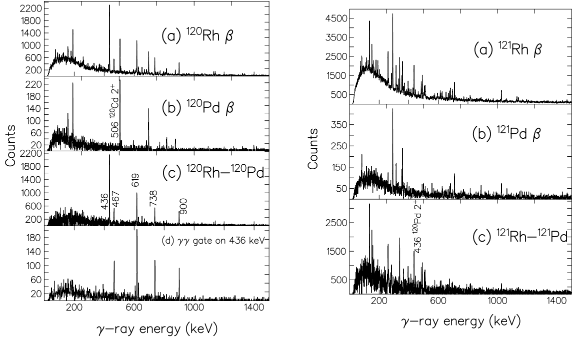
Figure 2: LEFT: Gamma-ray spectra associated with the decay of (a) ^{120}\text{Rh} and (b) ^{120}\text{Pd} . (c) A ^{120}\text{Pd} subtracted ^{120}\text{Rh} spectrum showing events associated with the primary decay of ^{120}\text{Rh} only, which are assumed to be gamma-ray transitions from excited states in the ^{120}\text{Pd} daughter nucleus. (d) Gamma-ray coincidence spectra gated on the 436 keV 2^+ \rightarrow 0^+ transition in ^{120}\text{Pd} . The \beta - \gamma correlation times for each of these spectra was 2.350 s.
