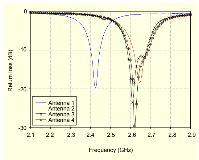
Fig. 3. Measured return loss characteristics for four different antennas.
