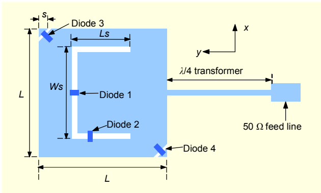
Fig. 1. Geometry of the proposed microstrip patch antenna with a U-slot.
