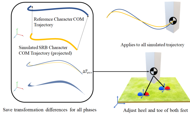
Figure 6: Conceptual depiction of aligning COM trajectory and calculating COM frame delta. The frames on the plane are the center of each foot and blue and red balls are its heel and toe contact points.
