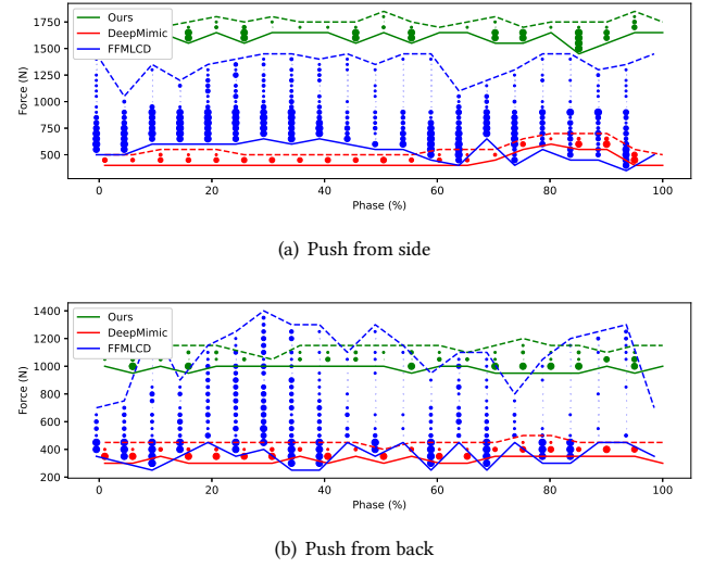
Figure 5: Plots for external pushes. Dotted line: the smallest external force at which the character always loses balance. Solid line: the largest external force at which the character maintains balance at each phase without falling. Circles: the ratio of successful balance maintenance (no falling within 20 seconds after the push) out of 10 trials at points where both balance maintenance and loss occur, with its size representing the proportion of successful balance maintenance.
