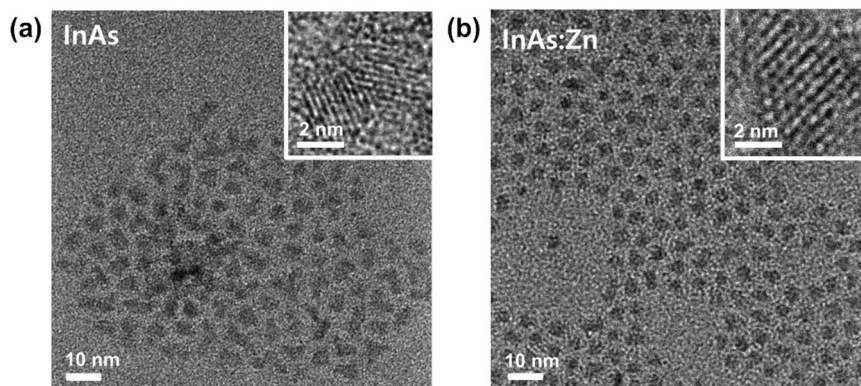
Fig. 4 Colloidal stability and size distribution of InAs and InAs:Zn QDs. TEM images of the InAs QDs made a without and b with the \text{ZnCl}_2 -TOP complex.
