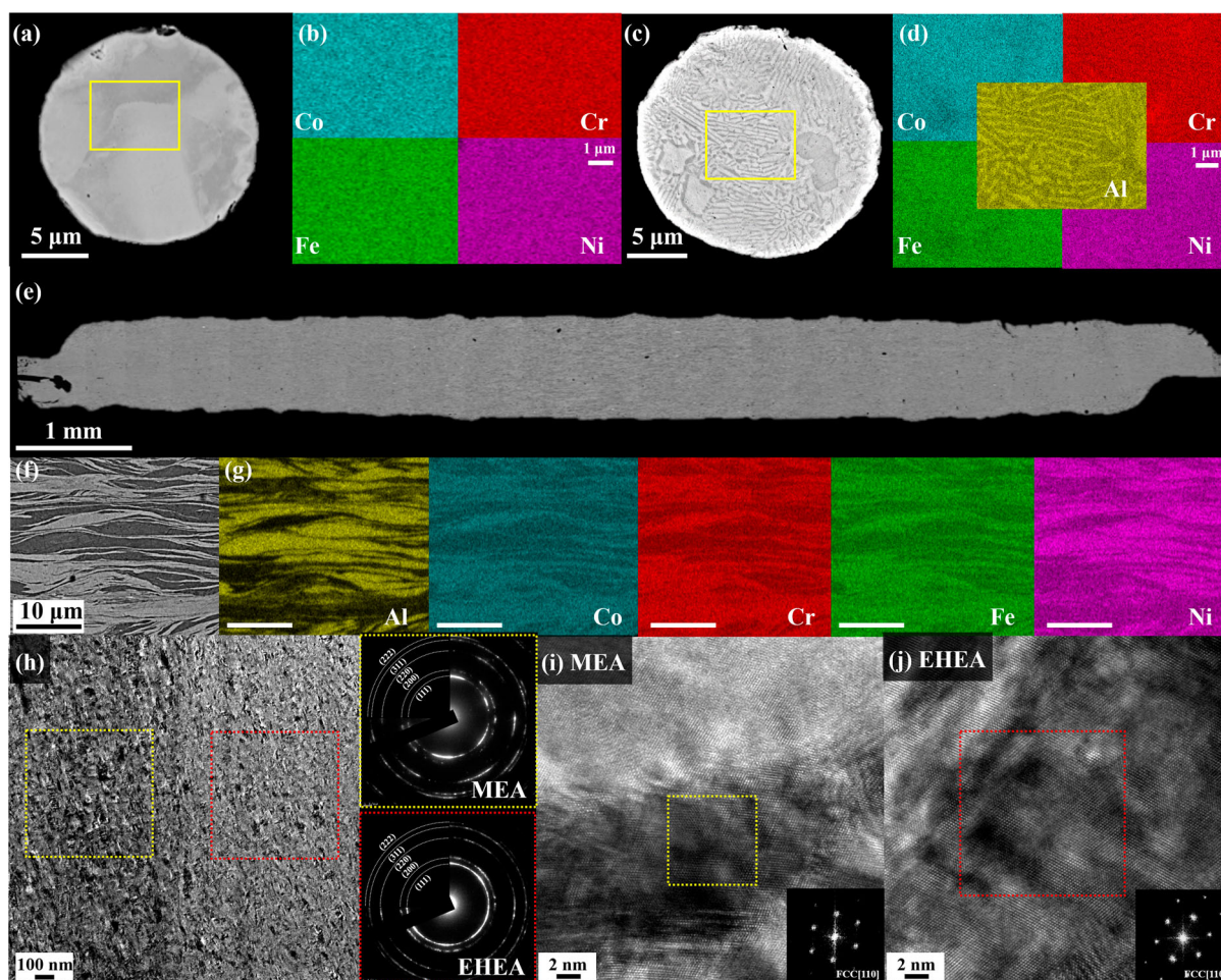
Figure 1. (a, c) SEM-BSE micrographs and (b, d) EDS maps of the gas-atomized (a, b) MEA powder and (c, d) EHEA powder, (e) the cross-section SEM image of the As-HPT sample, (f) SEM-BSE image of the As-HPT sample with (g) corresponding EDS maps, (h) bright field TEM micrographs of the MEA/EHEA interface with SAED ring patterns from MEA and EHEA regions, and HR-TEM micrographs of MEA and EHEA is shown in (i) and (j) accompanied by FFT patterns, respectively.
