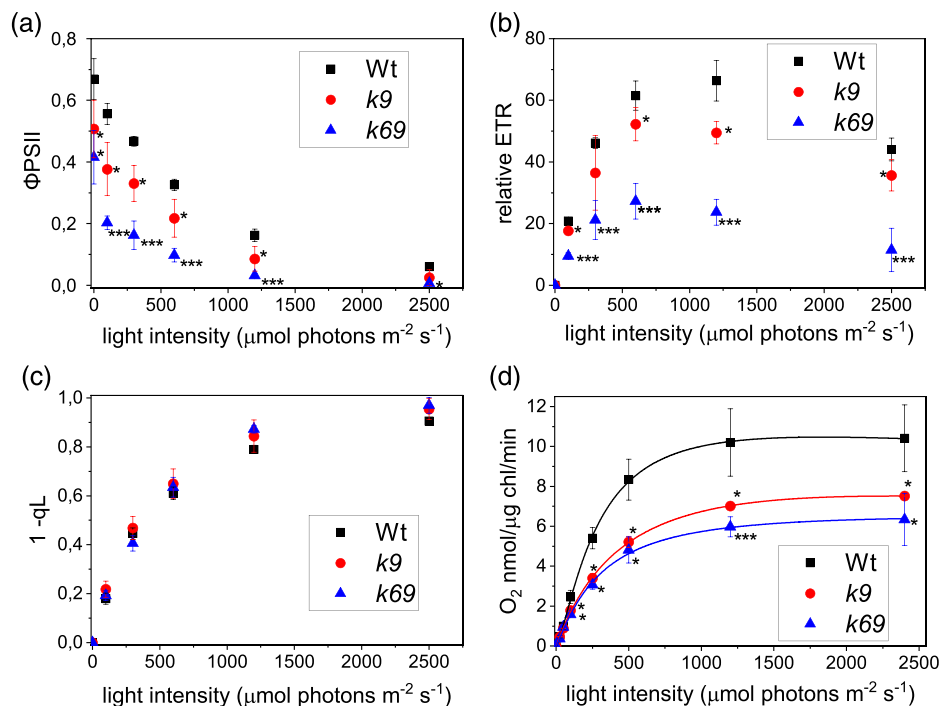
FIGURE 3 Characterization of the photosynthetic electron flow. Dependence of the (a) PSII operating efficiency ( \Phi_{\text{PSII}} ), (b) relative electron transport rate (ETR), (c) 1 - q_L (estimates the fraction of PSII centres with reduced Q_A ), and (d) photosynthetic \text{O}_2 evolution on actinic light intensity for wild type (Wt, black), k9 (red), and k69 (blue). Net photosynthetic rate data were fitted with Hill equation. Data are expressed as mean \pm SD. n > 3 . All data were collected from algae grown in high salts at 100\text{-}\mu\text{mol photons m}^{-2} \text{s}^{-1} . *Values that are significantly different (Student's t test, P < 0.05 ) from Wt. **Data that are significantly different between k6 and k69
