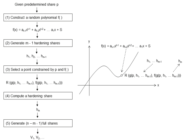
Fig. 5. Unconstrained Point Generation Technique to Generate Multiple Reinforcing Shares
