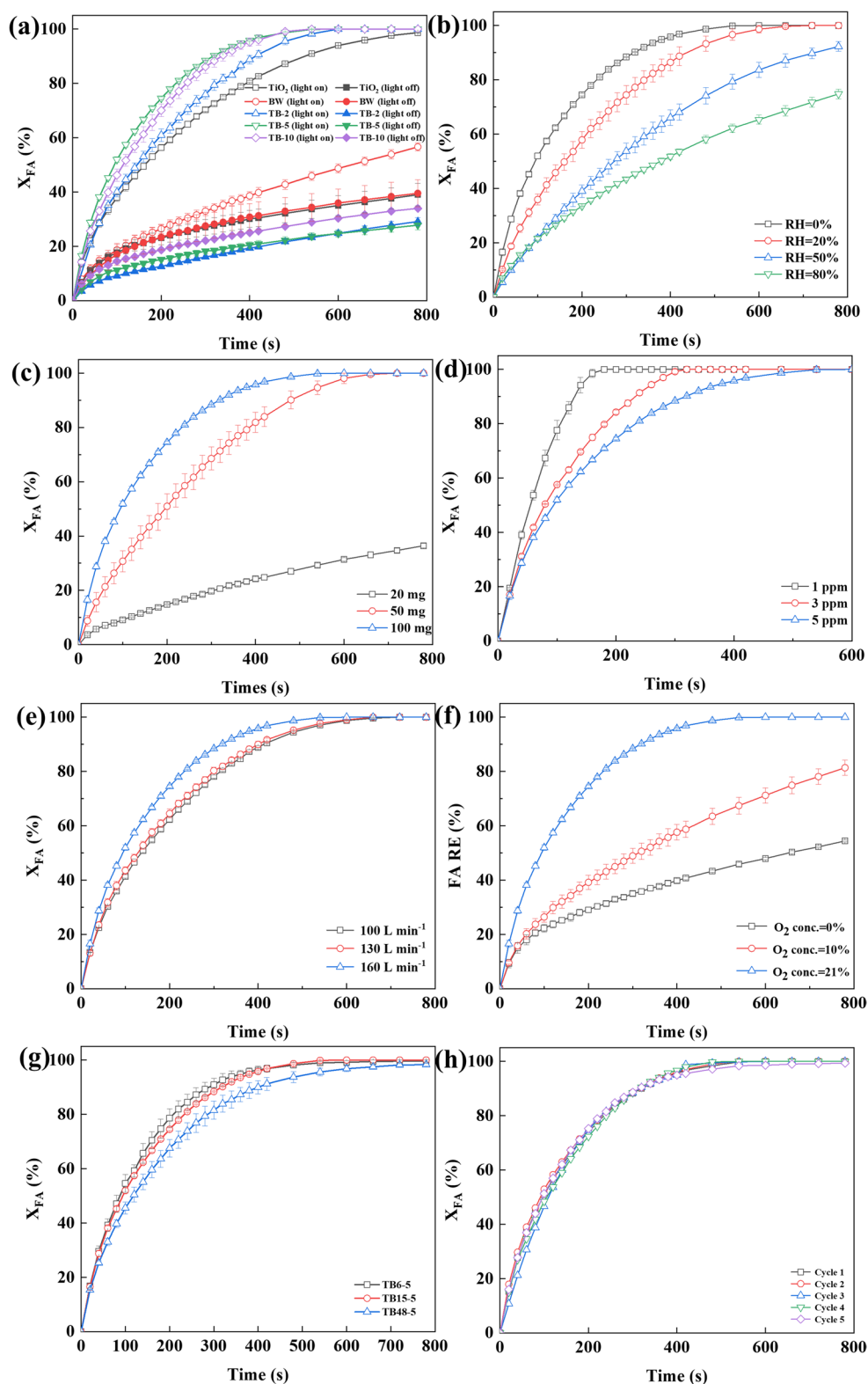
Fig. 8 Comparison of PCO efficiency ( X_{FA} ) of TB-x photocatalysts (base conditions: FA=5 ppm, m_{cat} =100 mg, flow rate=160 L min -1 , RH=0%, and O 2 concentration=21 vol%): (a) all photocatalysts prepared in this study, (b–g) tests under control of each process variable ((b) RH, (c) m_{cat} , (d) FA concentration, (e) AP flow rate, (f) O 2 concentration, (g) hydrothermal duration (6, 15, and 48 h)), and (h) tests over five cycles
