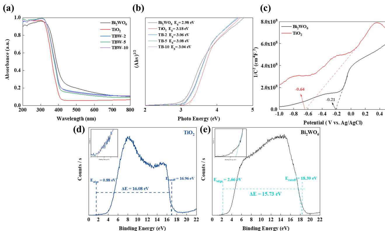
Fig. 4 Optoelectronic characterization of TB-x series catalysts along with the reference materials ( \text{Bi}_2\text{WO}_6 and \text{TiO}_2 ). (a) UV-vis spectra, (b) Tauc plots, (c) Mott-Schottky curves, (d) UPS spectra of \text{TiO}_2 , and (e) UPS spectra of \text{Bi}_2\text{WO}_6
