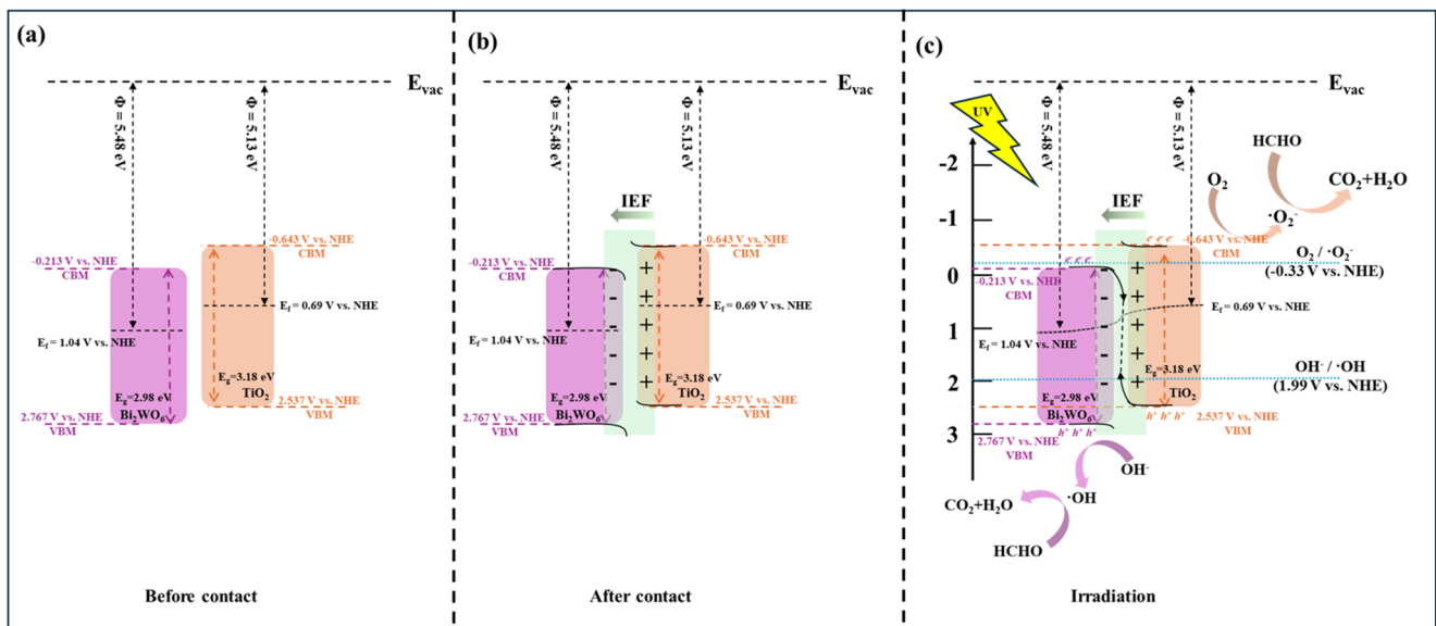
Fig. 5 Plot of S-scheme heterojunction and the associated charge transfer mechanism between \text{Bi}_2\text{WO}_6 (as OP) and \text{TiO}_2 (as RP): (a) before contact and (b-c) after contact [under (b) dark and (c) light irradiation conditions]
