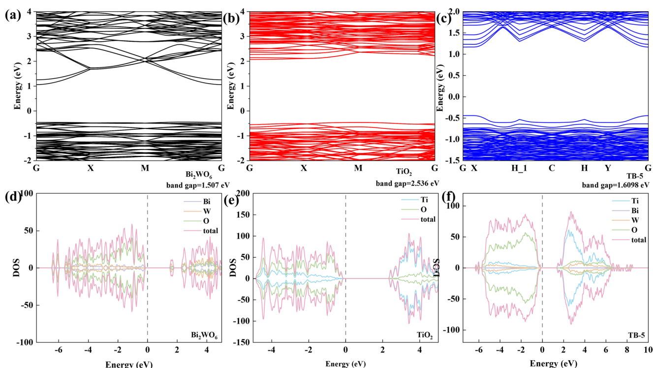
Fig. 10 Calculated band structures: (a) \text{Bi}_2\text{WO}_6 , (b) \text{TiO}_2 and (c) TB-5. DOS curves: (d) \text{Bi}_2\text{WO}_6 , (e) \text{TiO}_2 and (f) TB-5
