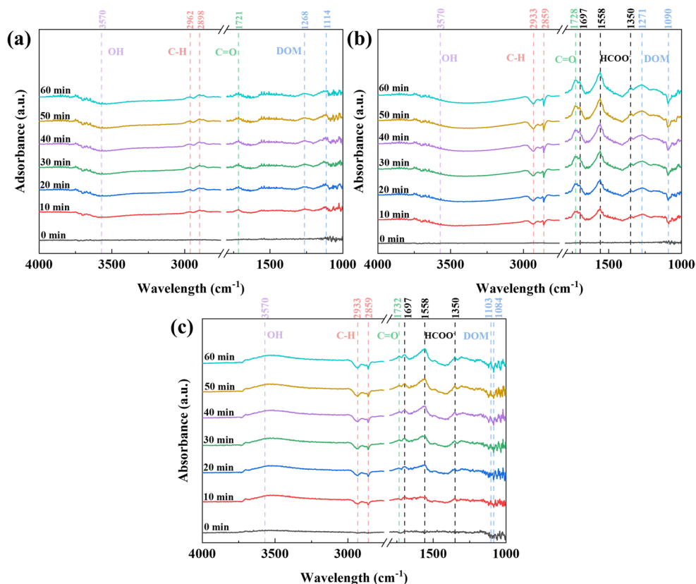
Fig. 9 In-situ DRIFTS spectra of TB-5 under different reaction conditions: (a) FA + air + UV off, (b) FA + air + UV on, and (c) FA + air + \text{H}_2\text{O} + UV on
