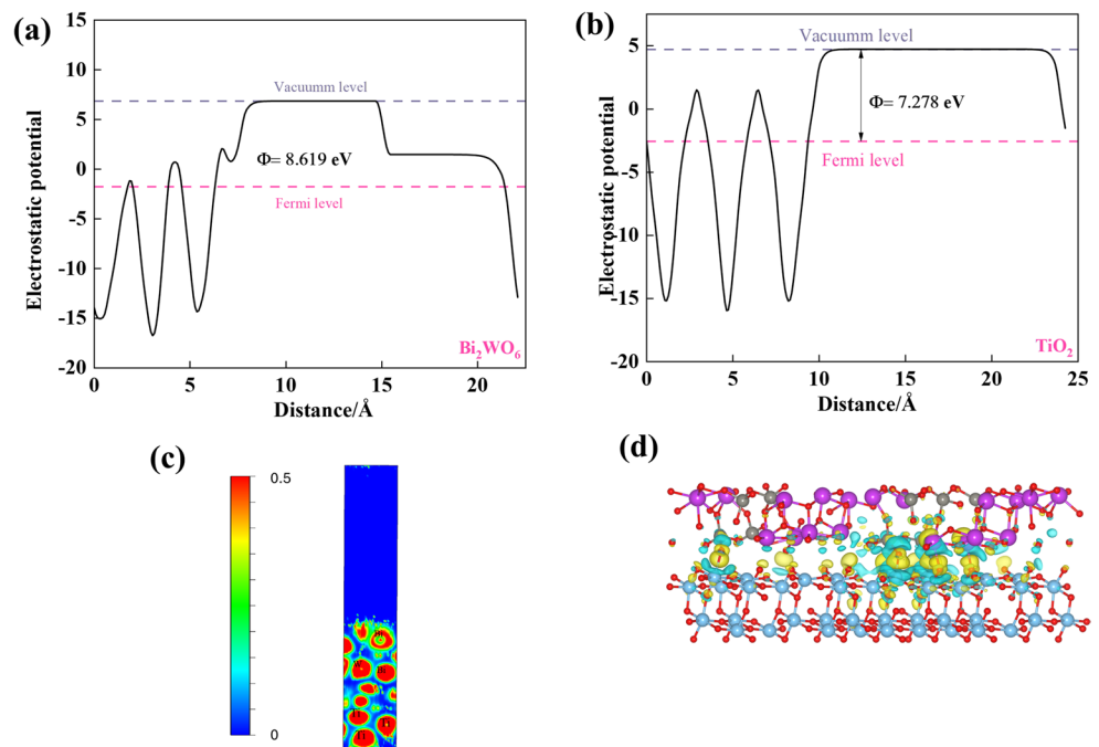
Fig. 11 Calculated work functions of (a) \text{Bi}_2\text{WO}_6 and (b) \text{TiO}_2 . (c) Electron localization function of TB-5 and (d) Charge density difference of TB-5 with an iso-surface of 0.002 e/Bohr 3
