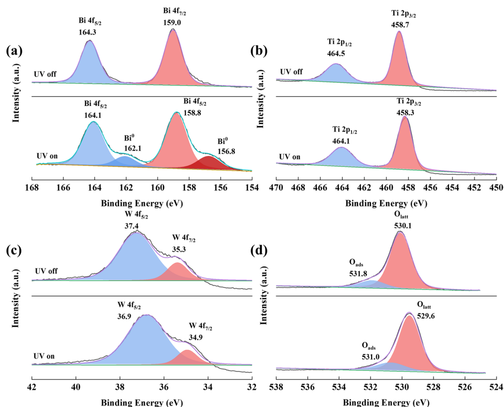
Fig. 6 In-situ XPS spectra of TB-5 under UV on/off conditions: (a) Bi 4f, (b) Ti 2p, (c) W 4f, and (d) O 1s
