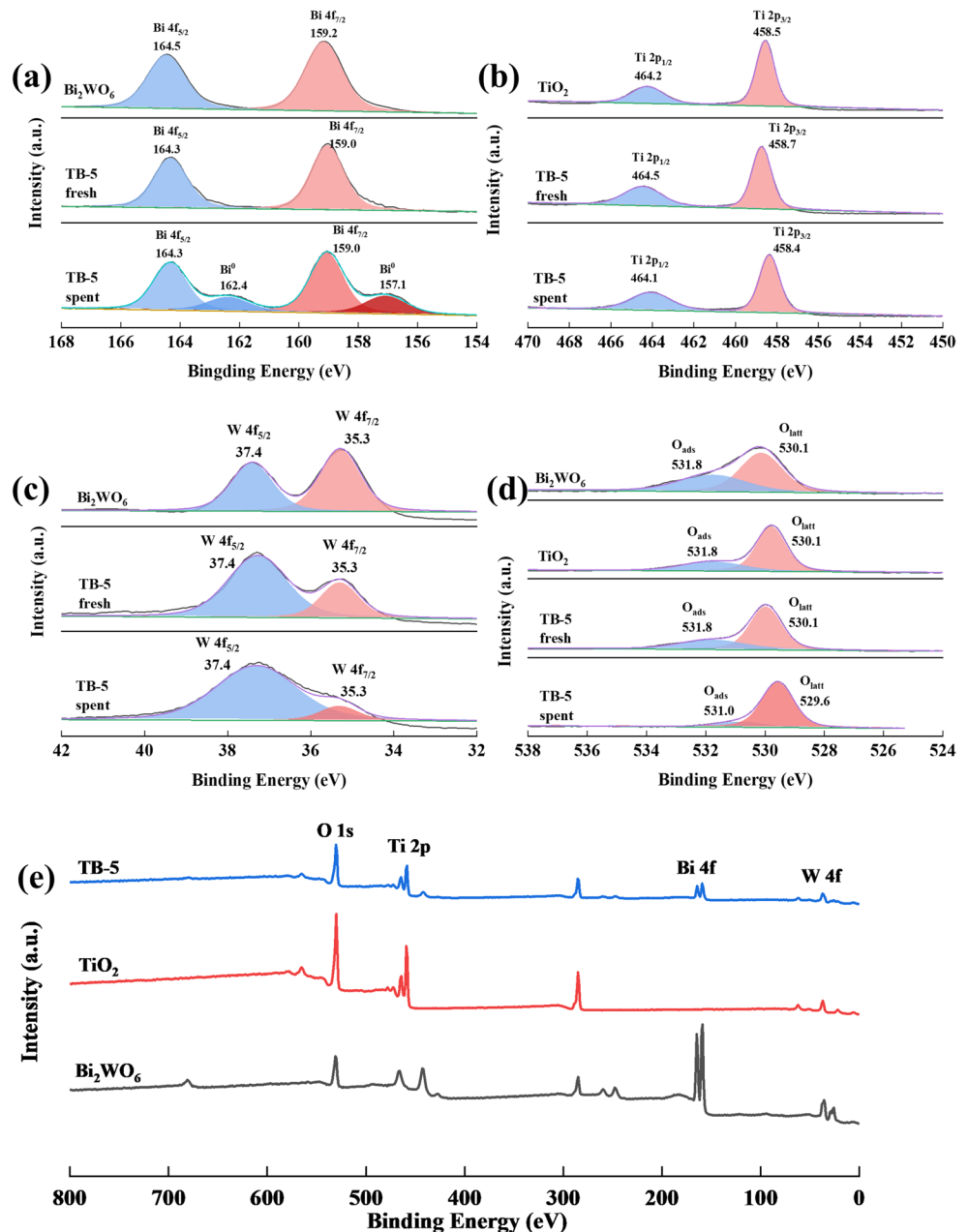
Fig. 3 XPS spectra of TB-5 along with the reference catalysts ( \text{Bi}_2\text{WO}_6 and \text{TiO}_2 ): (a) Bi 4f, (b) Ti 2p, (c) W 4f, (d) O 1s, and (e) full XPS spectra
