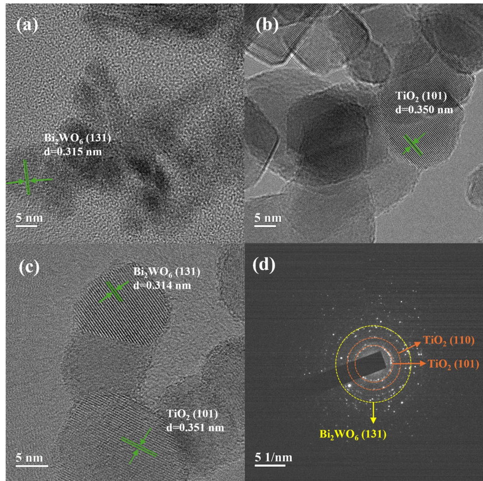
Fig. 1 TEM micrographs of the tested photocatalysts: (a) \text{Bi}_2\text{WO}_6 , (b) \text{TiO}_2 , (c) TB-5, and (d) SAED pattern of TB-5
